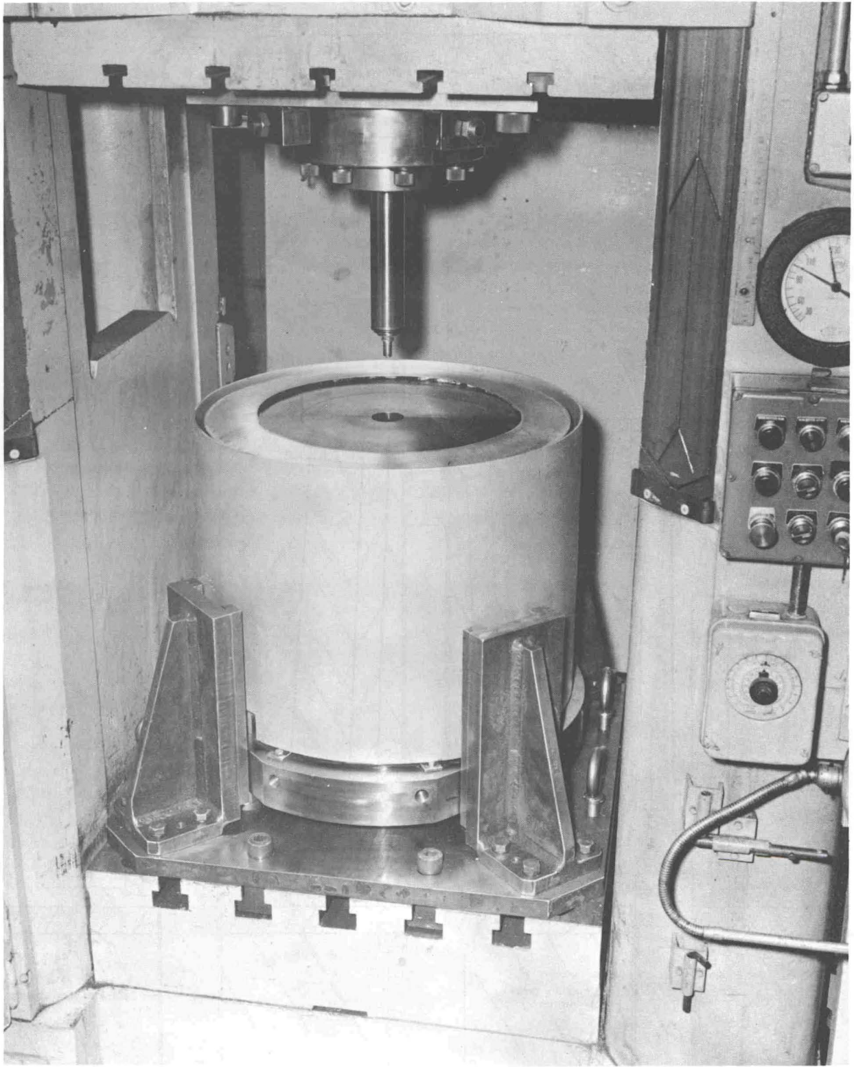
FIGURE 4. HYDROSTATIC-EXTRUSION TOOLING INSTALLED IN 700-TON VERTICAL HYDRAULIC PRESS AT BATTELLE
